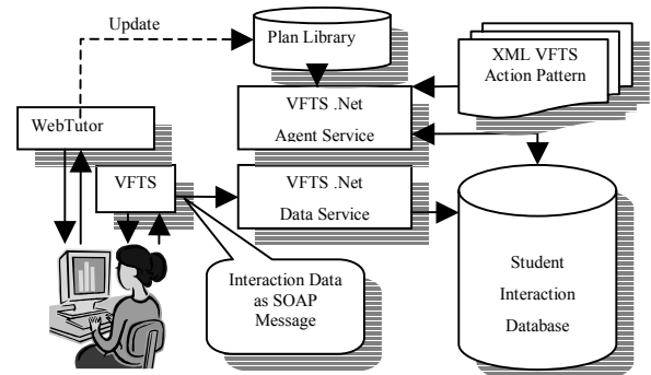
Figure 2: Plan recognition system in VFTS.
